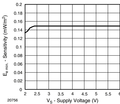
Fig. 14 - Sensitivity vs. Supply Voltage
