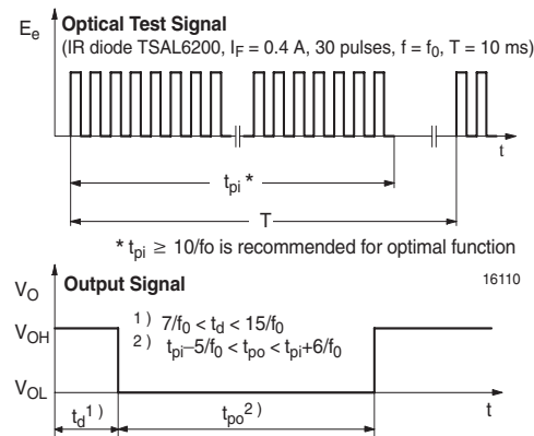
Figure 1. Output Function
