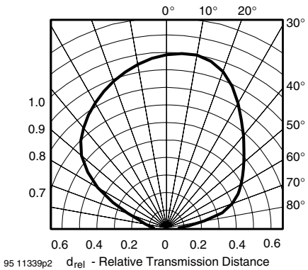
Figure 13. Vertical Directivity \varphi_y
