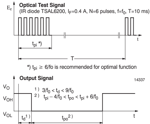
Figure 1. Output Function
