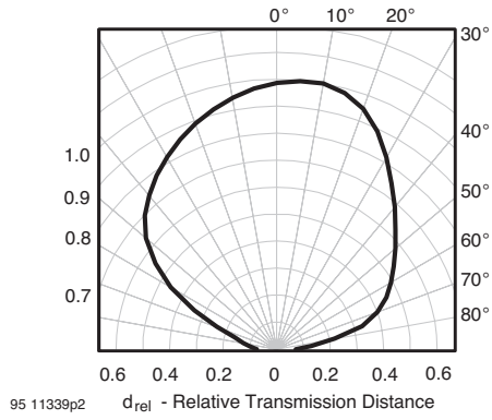
Figure 13. Vertical Directivity \varphi_y
