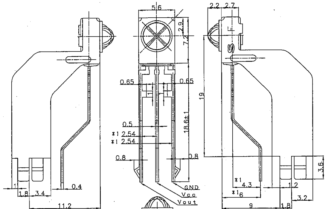
Example of mounting drawing from solder side(Reference)
