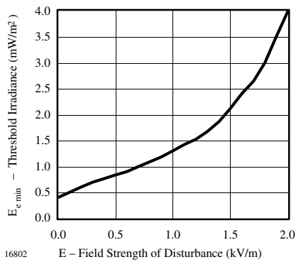
Figure 4. Threshold Irradiance vs. Field Strength of Disturbance
