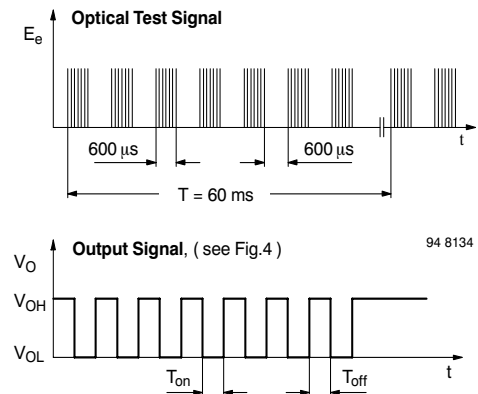
Figure 8. Output Function
