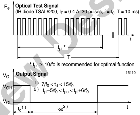
Figure 7. Output Function
