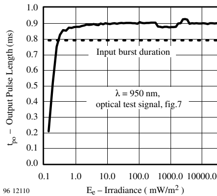
Figure 2. Sensitivity in Dark Ambient
