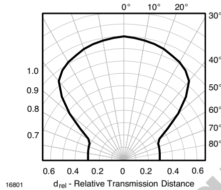
Figure 12. Directivity
