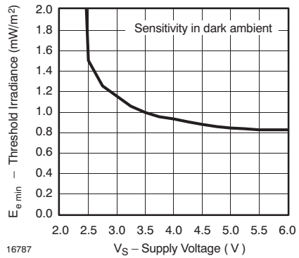
Figure 7. Sensitivity vs. Supply Voltage
