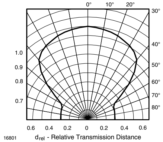
Fig. 12 - Horizontal Directivity
