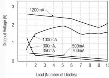
Dropout Voltage/Load
