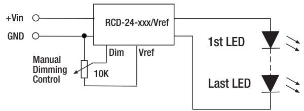
LED DIMMER for up to 10 white LEDs
