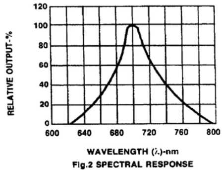
Fig.2 SPECTRAL RESPONSE
