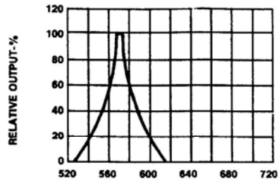
Fig.2 SPECTRAL RESPONSE
