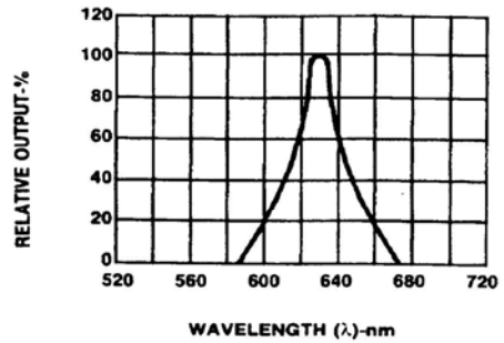
Fig.2 SPECTRAL RESPONSE
