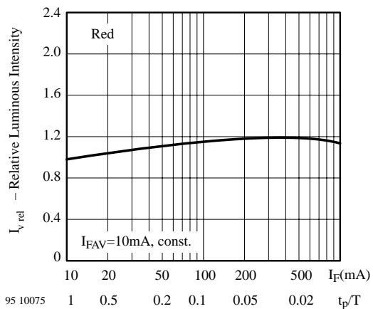
95 10075 I_F (mA) Figure 6. Rel. Lumin. Intensity vs. Forw. Current/Duty Cycle
