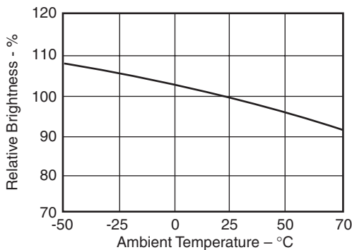
Fig. 1C. Relative Luminous Intensity vs. Temperature (See Note 2)
