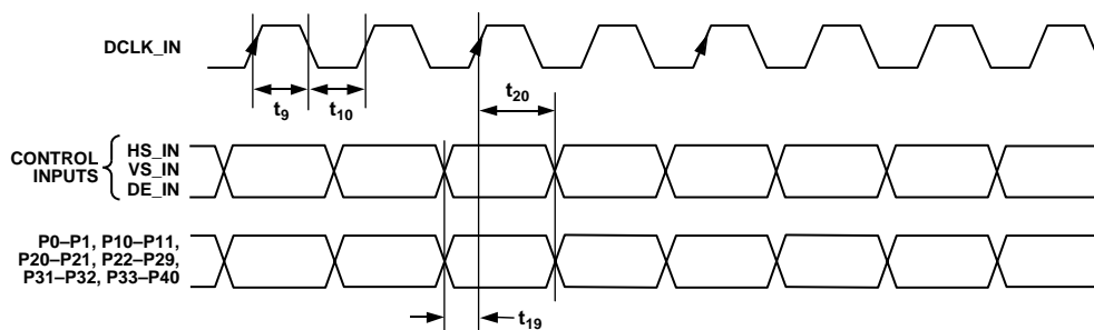
Figure 8. Digital Input Port and Control Input Timing
