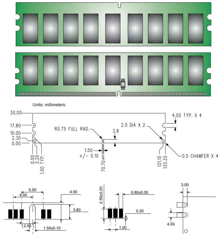
Figure 1: KVR800D2E5/2GI 240-Pin DIMM
