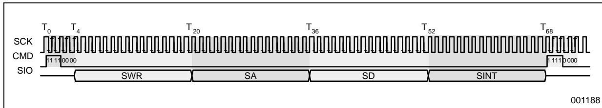
Figure 4-9. MSIO Register Write Transaction
