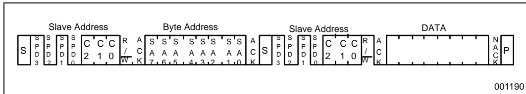
Figure 4-11. Random Byte Read Timing
