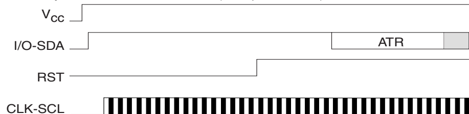
Figure 2. Asynchronous T = 0 Protocol (Gemplus Patent)
