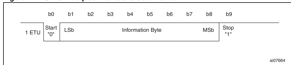
Figure 4. SRT512 request frame character format
