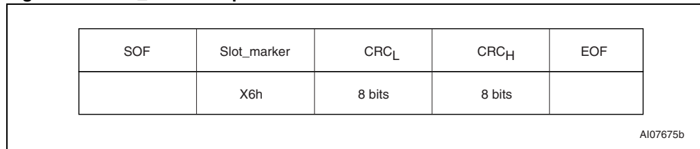
Figure 28. Slot_marker request format
