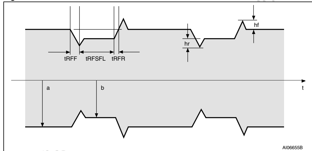
Figure 4. 10% modulation waveform
