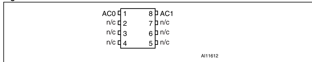
Figure 2. UDFPN8 connections
