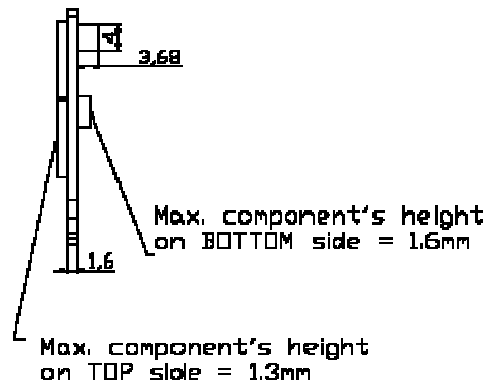
Figure 4: uSSD 2x5 Low Profile Version
