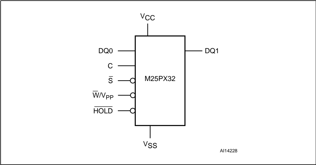
Figure 1. Logic diagram
