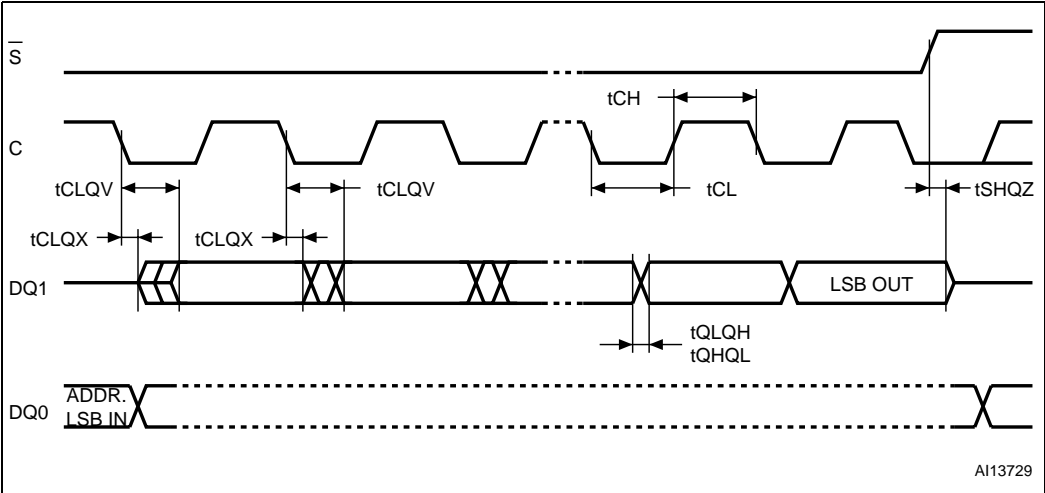
Figure 34. Output timing
