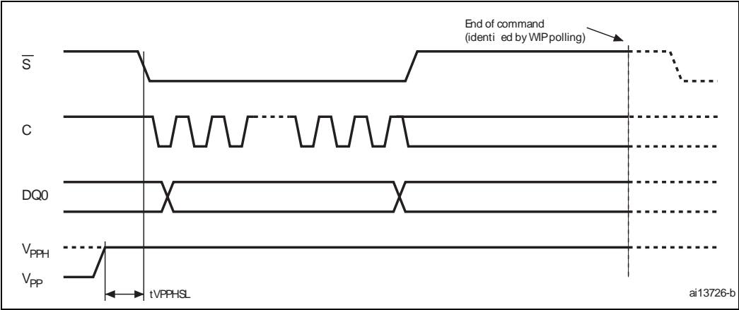
Figure 35. V_{PPH} timing
