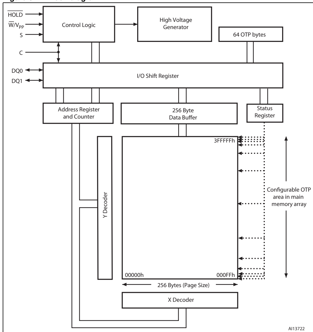
Figure 8. Block diagram
