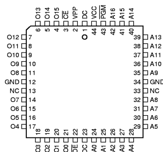
PLCC Top View
