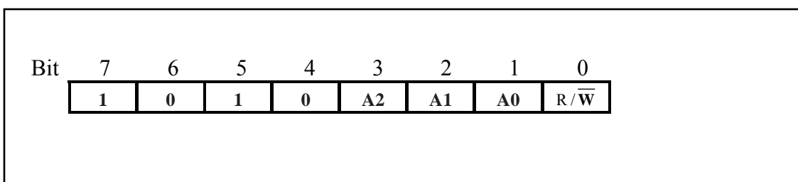
Fig. 5: Slave Address
