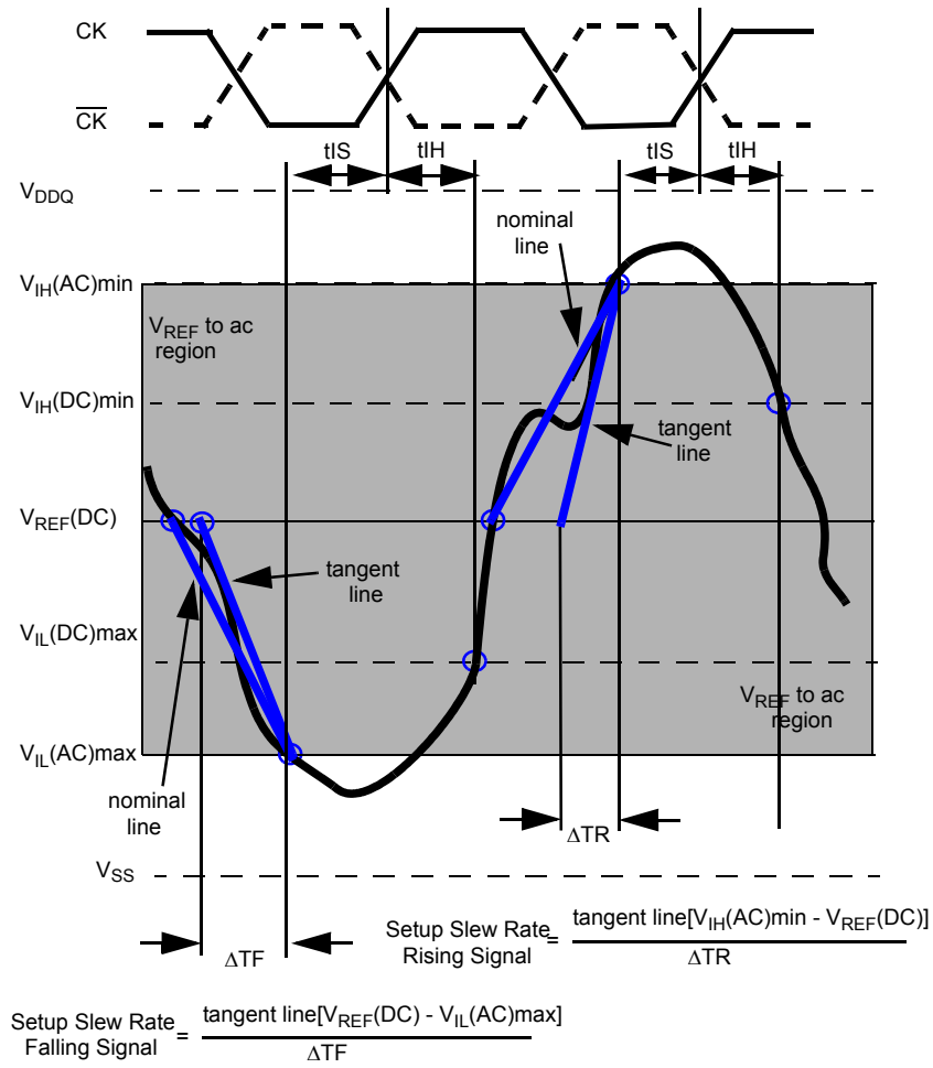
Figure 14 - Illustration of tangent line for t IS
