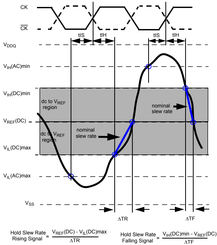
Figure 15 - Illustration of nominal slew rate for tIH
