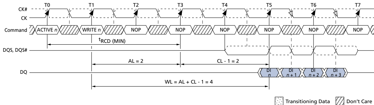
Figure 39: WRITE Latency
