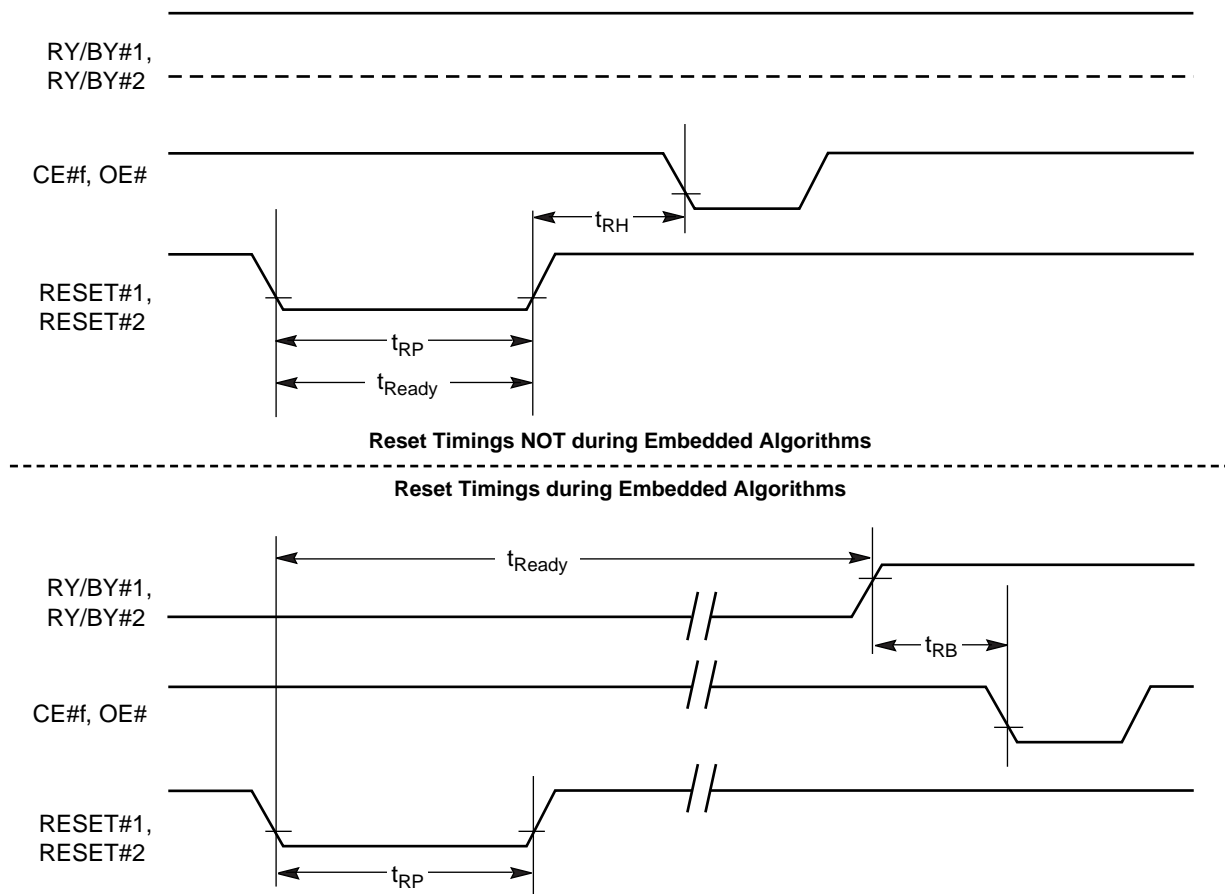
Figure 16. Reset Timings
