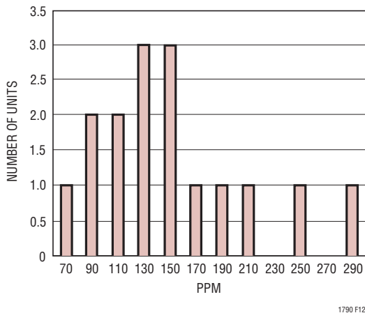
Figure 12. 3X IR Reflow Peak Temperature = 250°C, Delta Output Voltage (ppm)
