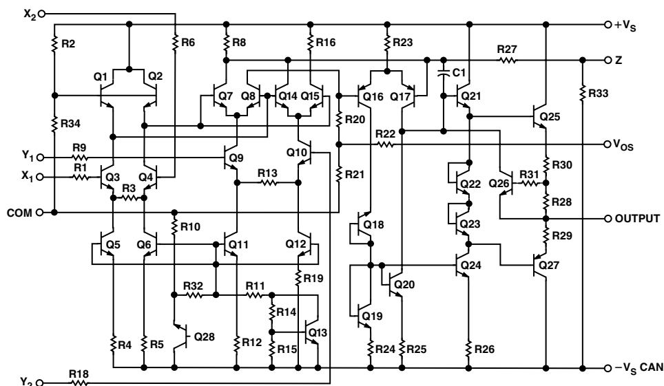
Figure 2. Schematic Diagram
