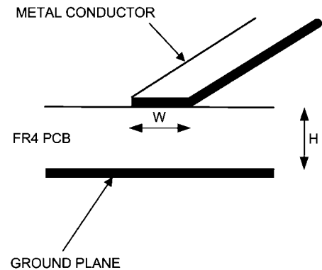
FIGURE 15. Microstrip Configuration
