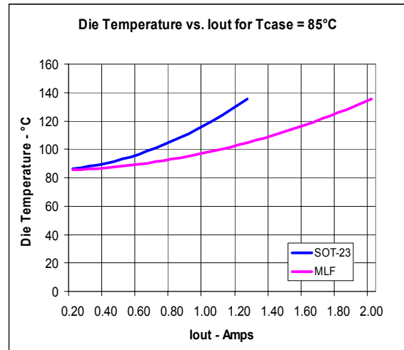
Figure 10. Die Temperature vs. I OUT
