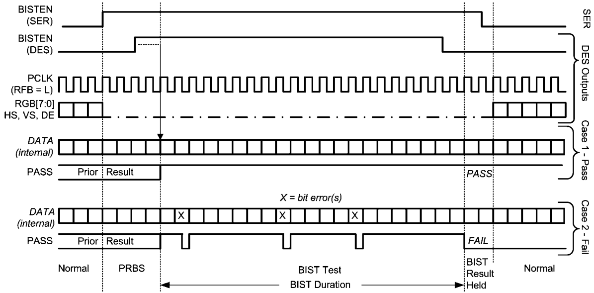
FIGURE 29. BIST Waveforms
