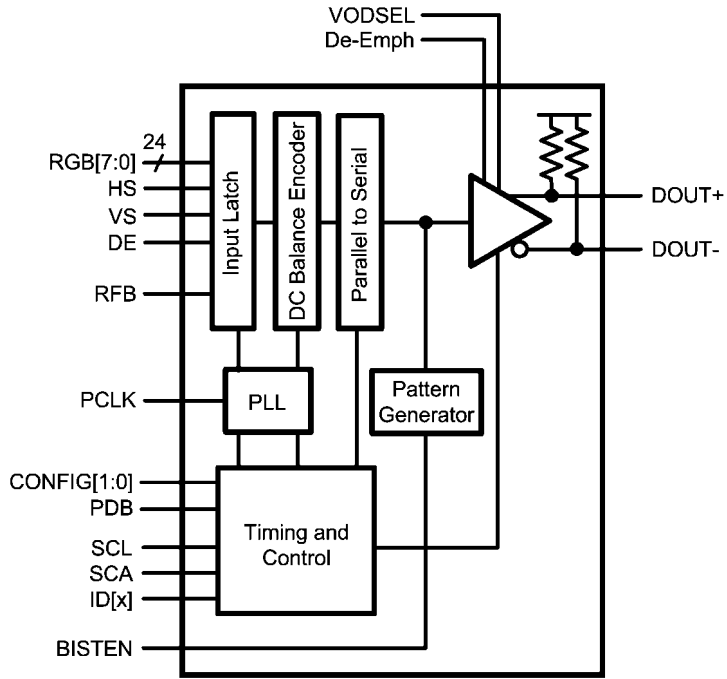
DS90UR905Q - SERIALIZER
