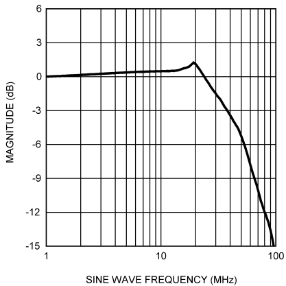
FIGURE 6. Bandwidth
