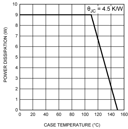
FIGURE 11. Power Derating Curve
