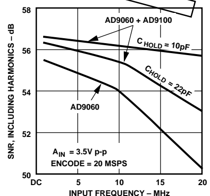
SNR vs. Analog Input
