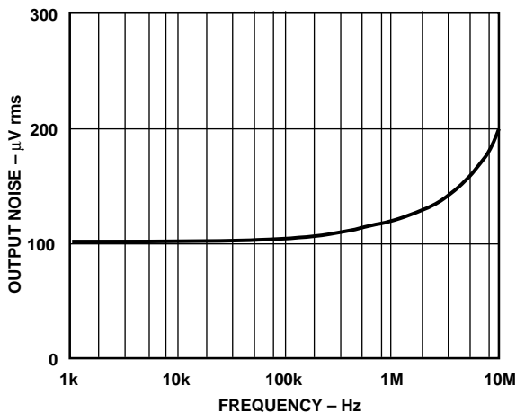
Figure 4. RMS Noise vs. Input Bandwidth of ADC
