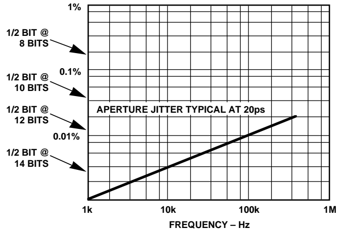
Figure 5. Error Magnitude vs. Frequency
