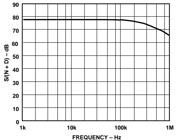
Figure 7. Signal/(Noise and Distortion) vs. Frequency
