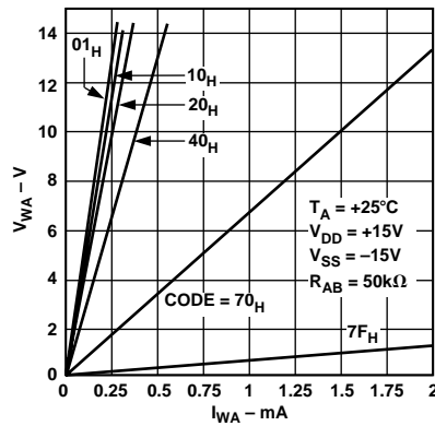
Figure 6. Resistance Linearity vs. Conduction Current
