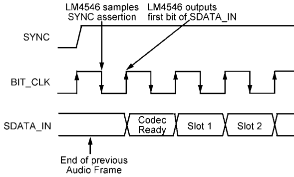
FIGURE 7. Start of Audio Input Frame
