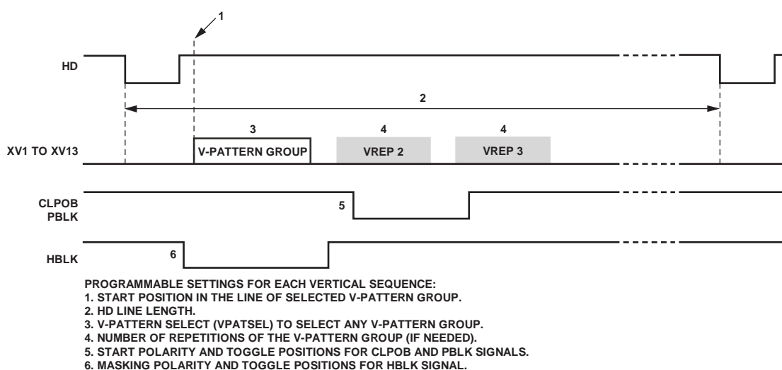
Figure 37. V-Sequence Programmability
