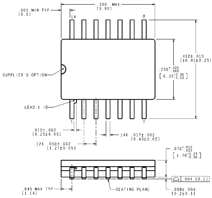
MIL-PRF-38535 CONFIGURATION CONTROL CONTROLLING DIMENSION IS INCH VALUES IN [ ] ARE MILLIMETERS DIMENSIONS IN ( ) FOR REFERENCE ONLY WG14A (Rev D) SAMPLE TEXT 14-Pin Ceramic Package (WG) NS Package Number WG14A
