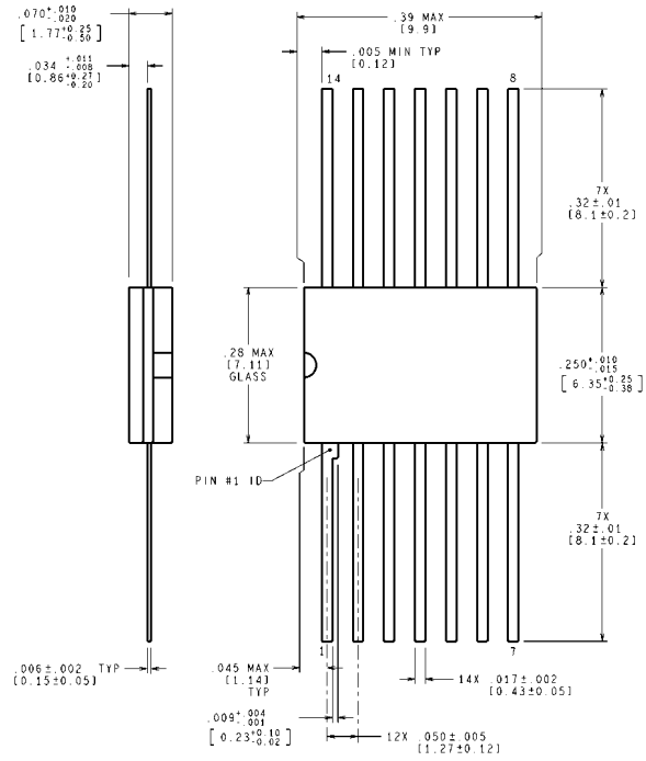
MIL-PRF-38535 CONFIGURATION CONTROL MIL-STD-1835B CONFIGURATION CONTROL CONTROLLING DIMENSION IS INCH VALUES IN [ ] ARE MILLIMETERS W14B (Rev P) SAMPLE TEXT Ceramic Flatpak Package NS Package Number W14B
