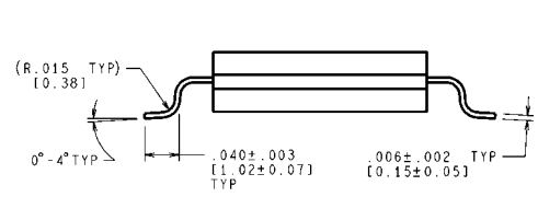
MIL-PRF-38535 CONFIGURATION CONTROL CONTROLLING DIMENSION IS INCH VALUES IN [ ] ARE MILLIMETERS DIMENSIONS IN ( ) FOR REFERENCE ONLY WG14A (Rev D) SAMPLE TEXT 14-Pin Ceramic Package (WG) NS Package Number WG14A
