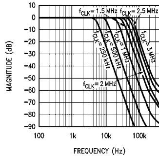
TL/H/10557-14 FIGURE 5b. LMF40-50 Amplitude Response with \pm 5V Supplies
