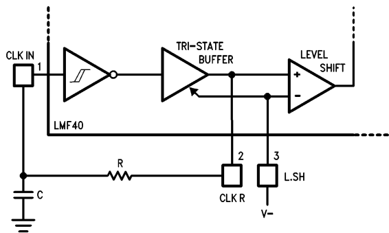
TL/H/10557-7 FIGURE 1. Schmitt Trigger R/C Oscillator
