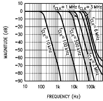
TL/H/10557-13 FIGURE 5a. LMF40-100 Amplitude Response with \pm 5V Supplies
