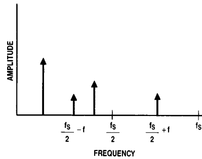
(b) Output Signal Spectrum. Note that the input signal at \frac{f_s}{2} + f causes an output signal to appear at \frac{f_s}{2} - f .
