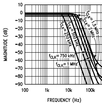
TL/H/10557-16 FIGURE 5d. LMF40-50 Amplitude Response with \pm 2.5V Supplies
