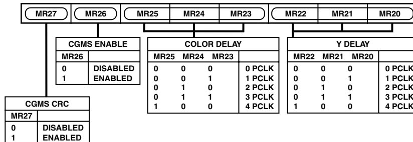
Figure 22. Mode Register 2
