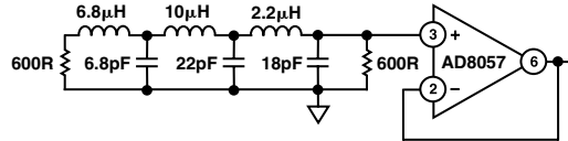
Figure 59. Example for Output Filter: PS Mode/ 2x Oversampling
