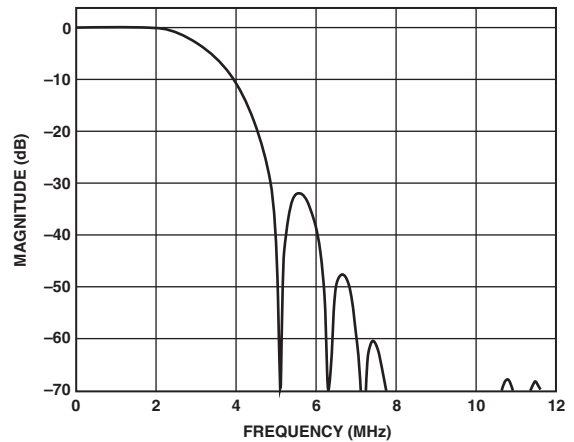
TPC 18. Chroma 3.0 MHz LP Filter
