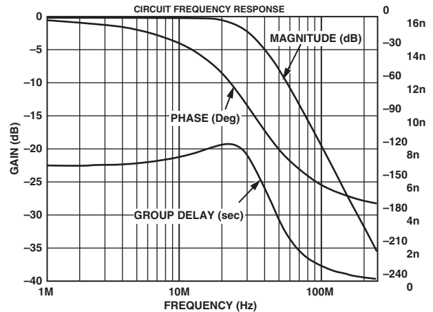
Figure 55. Filter Plot for Output Filter for SD, 16 \times Oversampling
