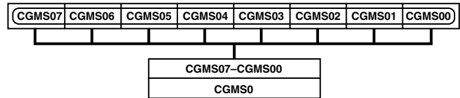
Figure 32. CGMS0 Data Register
