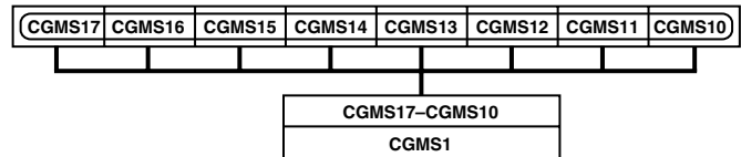
Figure 31. CGMS1 Data Register
