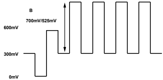
Figure 129. HD RGB Output Levels—RGB Sync Enabled
