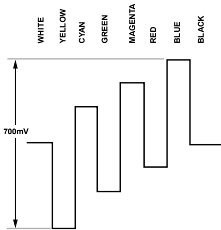
Figure 118. Pb Levels—NTSC
