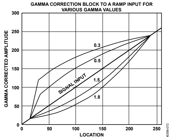
Figure 71. Signal Input (Ramp) and Selectable Output Curves
