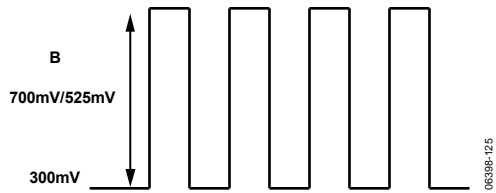
Figure 126. SD/ED RGB Output Levels—RGB Sync Disabled
