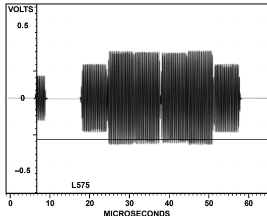
Figure 134. PAL Luma
