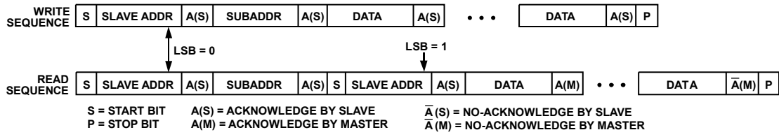
Figure 50. I 2 C Read and Write Sequence
