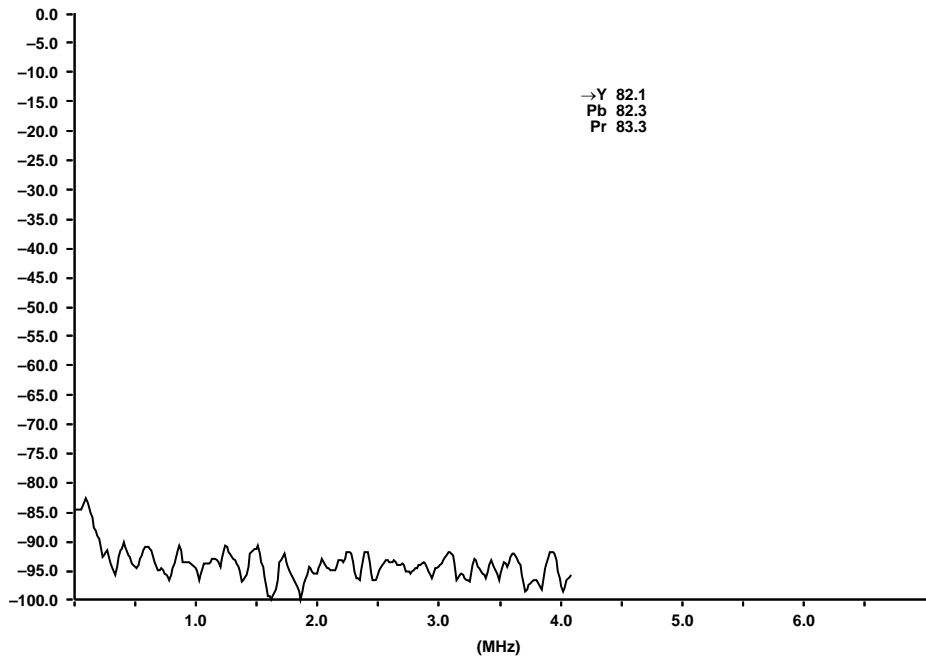
Figure 99. PAL YUV SNR Plot
