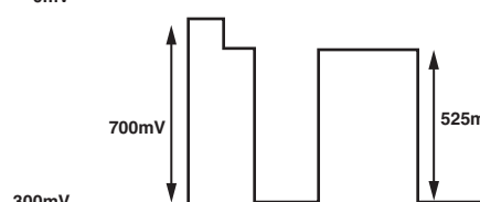
Figure 98. SD RGB Output Levels—RGB Sync Enabled
