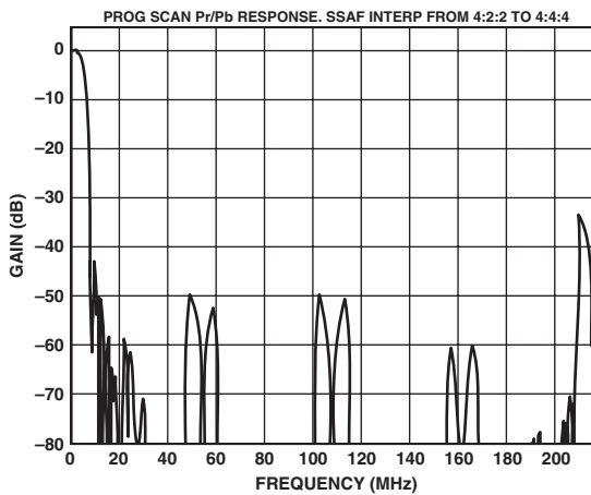
TPC 2. PS—UV 8x Oversampling Filter (SSAF)
