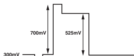
Figure 97. SD RGB Output Levels—RGB Sync Disabled
