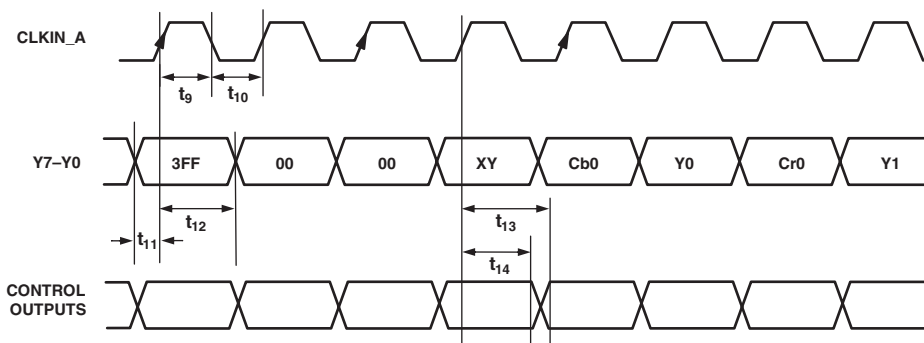
Figure 6. PS Only 4:2:2 1x8-Bit Interleaved at 27 MHz EAV/SAV Input Mode [Input Mode 100]
