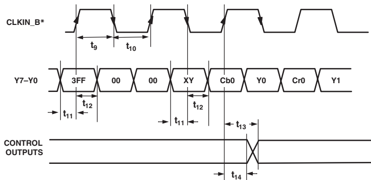
Figure 5. PS 4:2:2 1x8-Bit Interleaved at 54 MHz HSYNC/VSYNC Input Mode [Input Mode 111]
