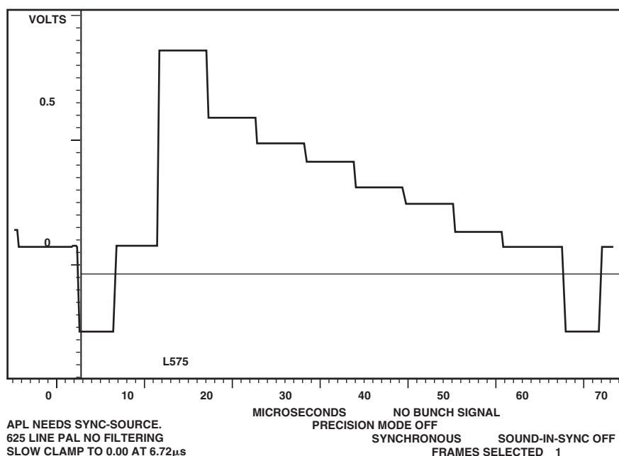
Figure 110. PAL Luma
