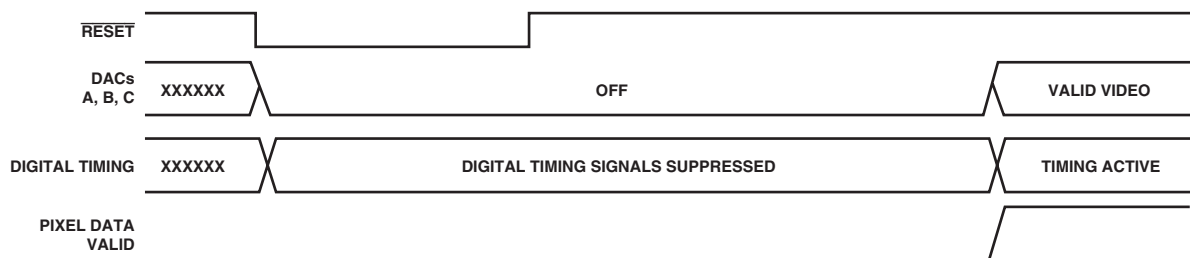
Figure 32. \overline{\text{RESET}} Timing Sequence
