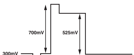
Figure 95. PS RGB Output Levels
