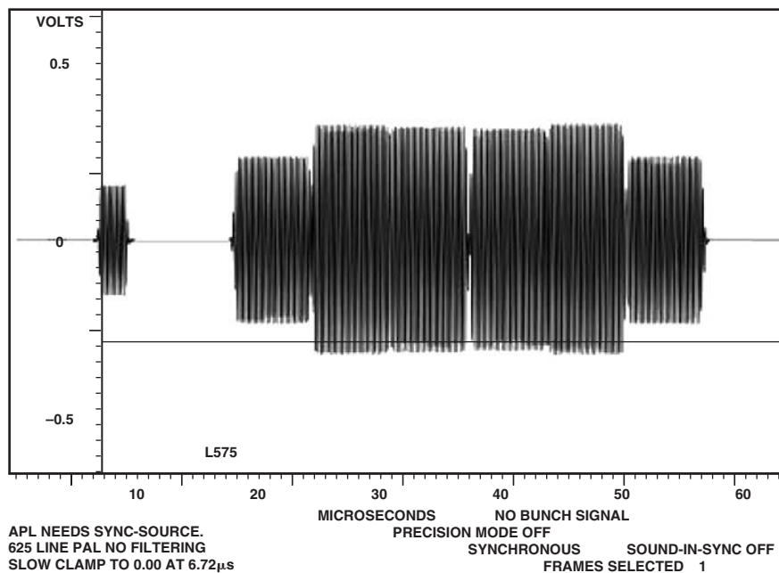
Figure 109. PAL Chroma
