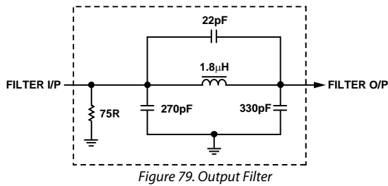
Figure 79. Output Filter
