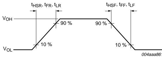
Fig 29. Rise time and fall time
