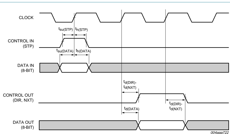
Fig 33. ULPI interface timing
