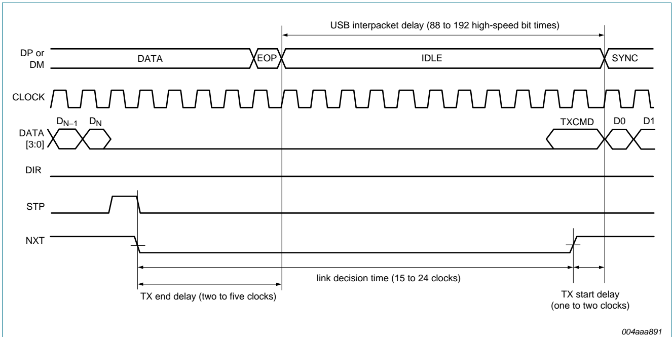
Fig 13. High-speed transmit-to-transmit packet timing
