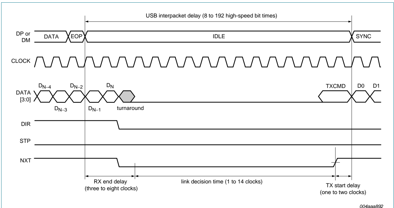
Fig 14. High-speed receive-to-transmit packet timing
