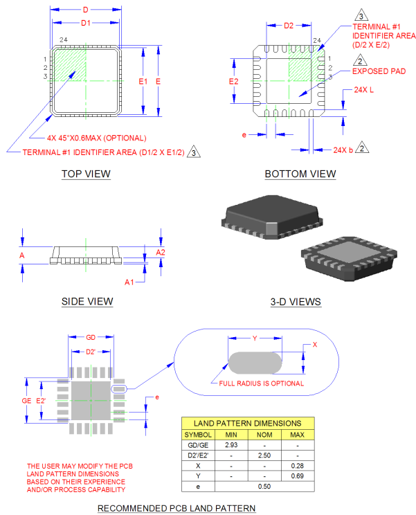
Figure 4.1 24-pin QFN, 4x4mm Body, 0.5mm Pitch
