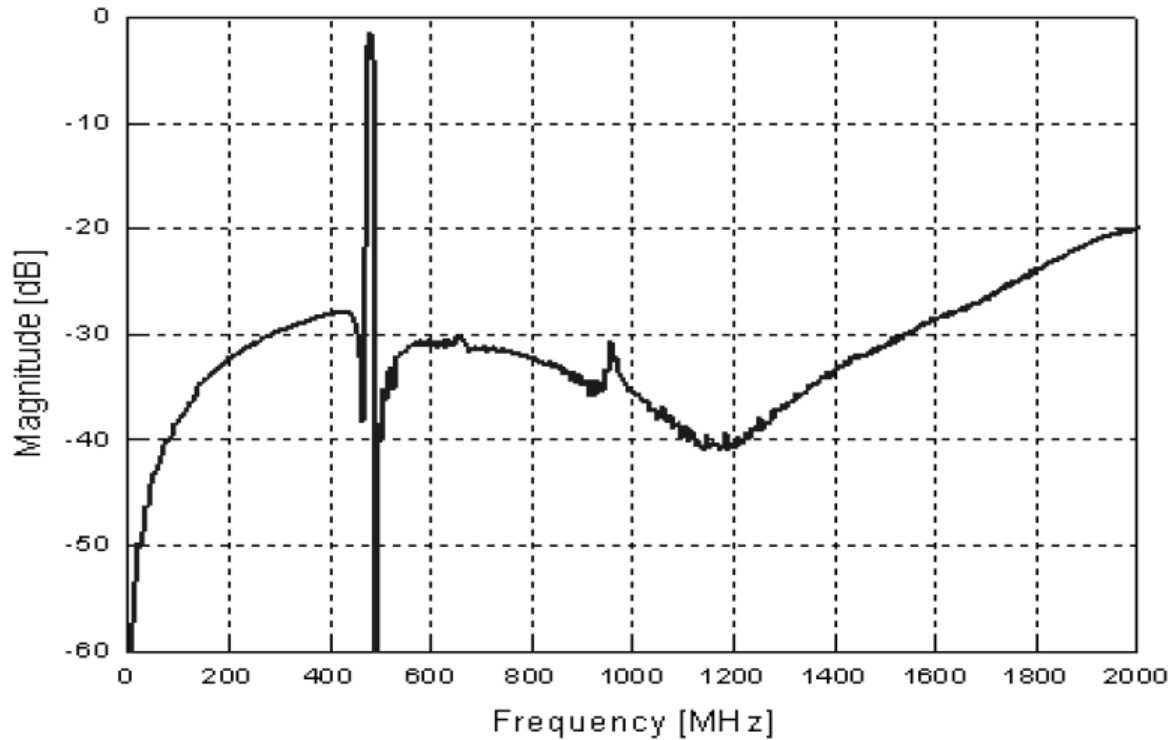
Passband Plot
