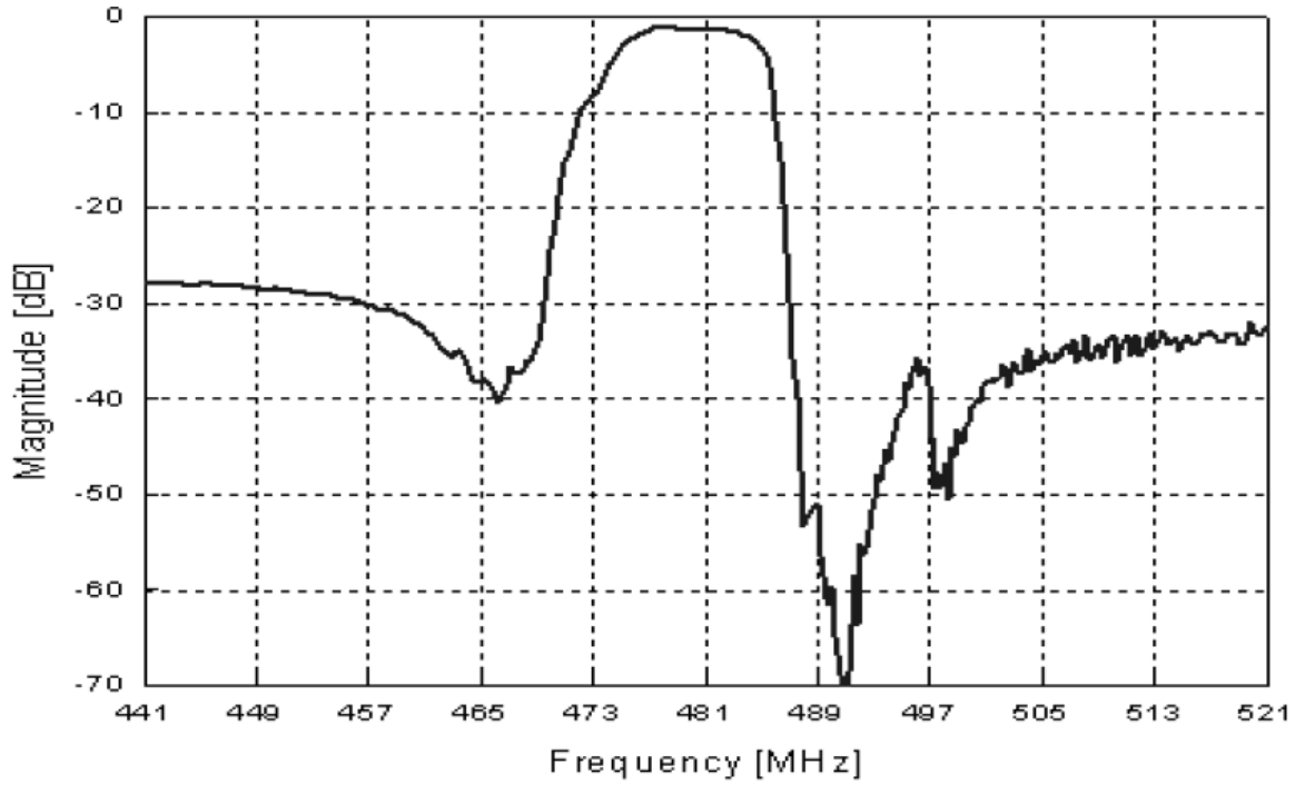
Passband Plot
