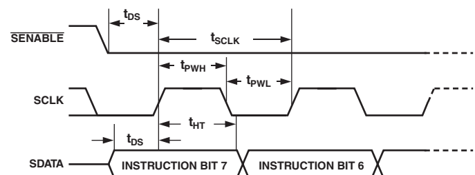
Figure 5. Timing Diagram Register Write to AD9975
